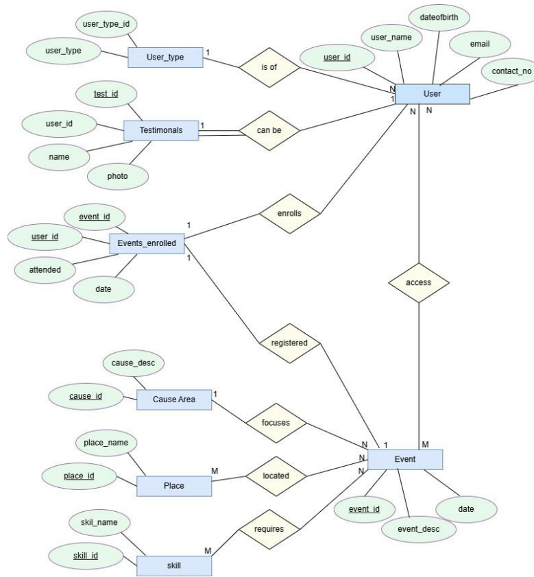
Fig 3 ER Diagram of the project
