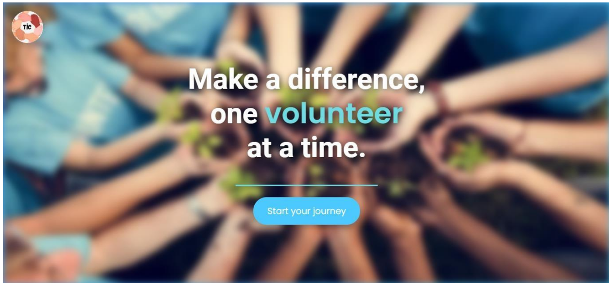
Fig 5.1 Home page
